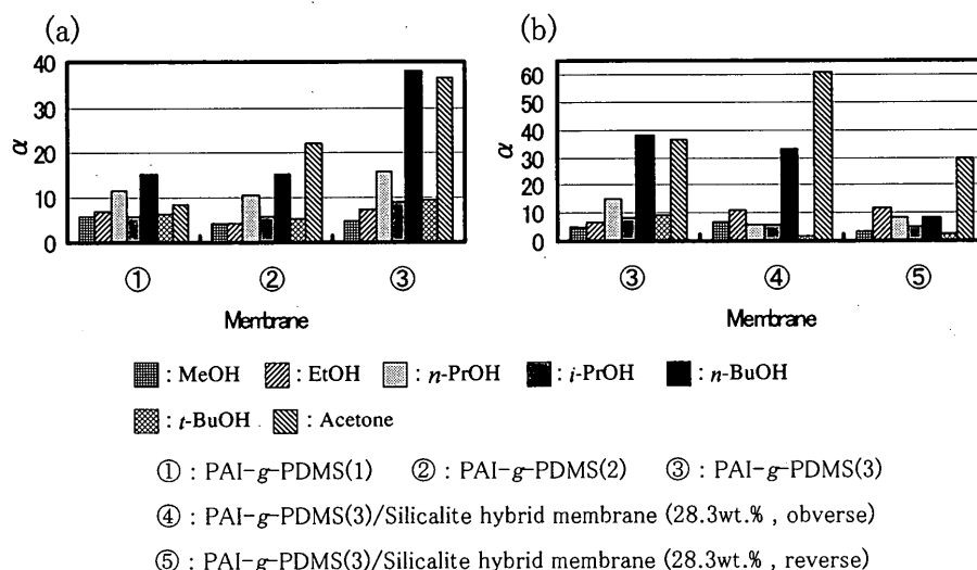
Fig. 1 Comparisons of separation factors in the pervaporation organic liquids/water mixtures through PAI- g -PDMS (1)~(3) membranes and PAI- g -PDMS/silicalite hybrid membrane.
