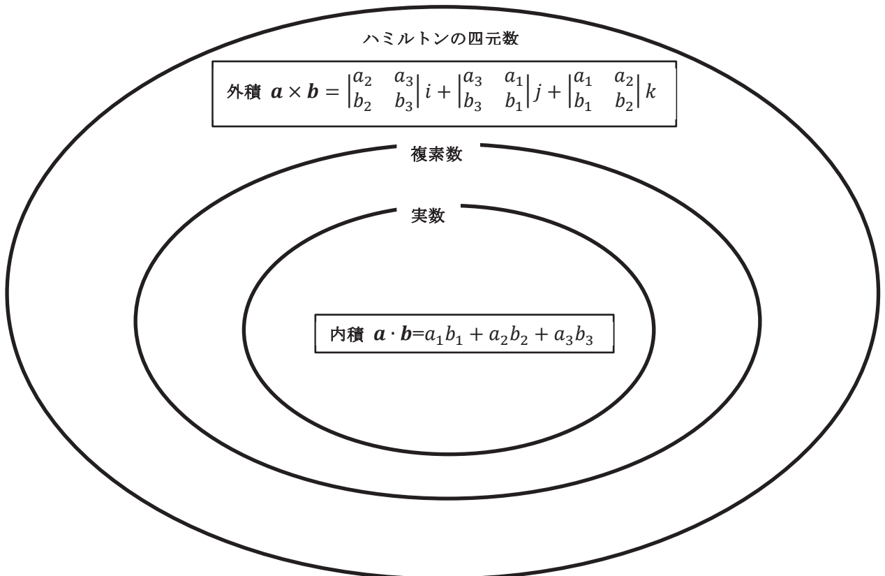
Fig.1 set inclusion relation
