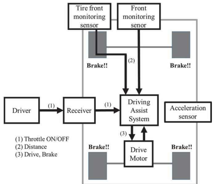
Fig. 4 Experiment equipment.
