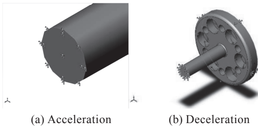
Fig. 8 Fixed conditions in fatigue structure analysis.
