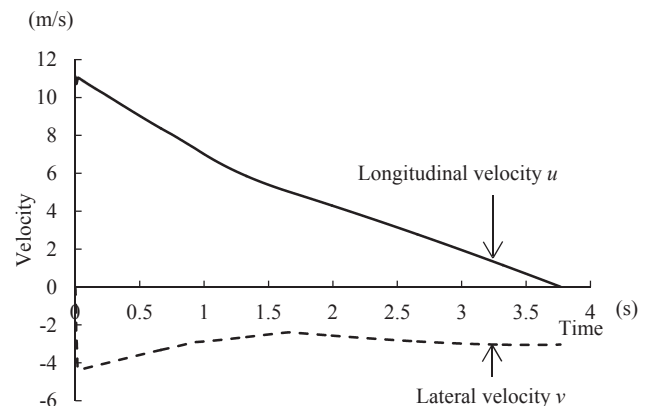
Fig. 13 Comparison time change of longitudinal velocity and lateral velocity
