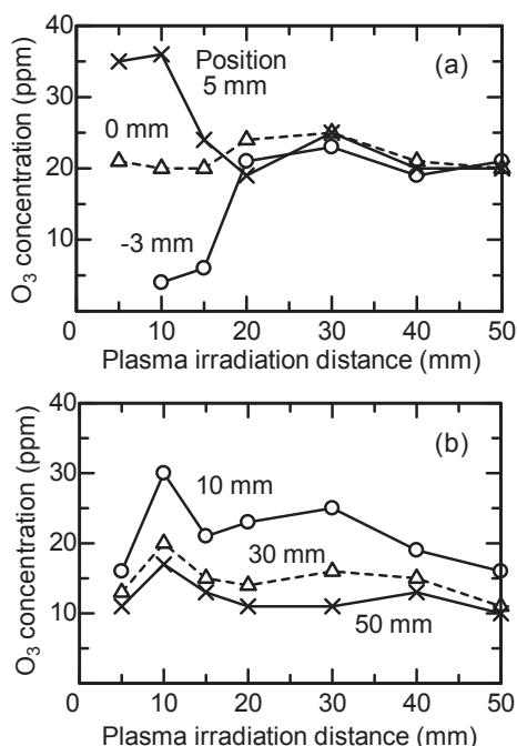
Fig. 6 Dependence of O 3 concentration on irradiation distance; (a) short and (b) long measurement positions (applied voltage 10 kV, gas flow rate 10 L/min).
