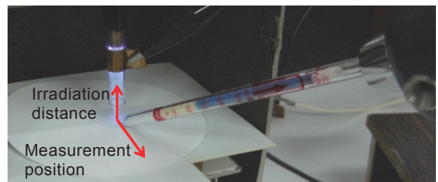
Fig. 3 Experiment for measuring O 3 concentration (Irradiation distance 5~50 mm, Measurement position -3~50 mm).
