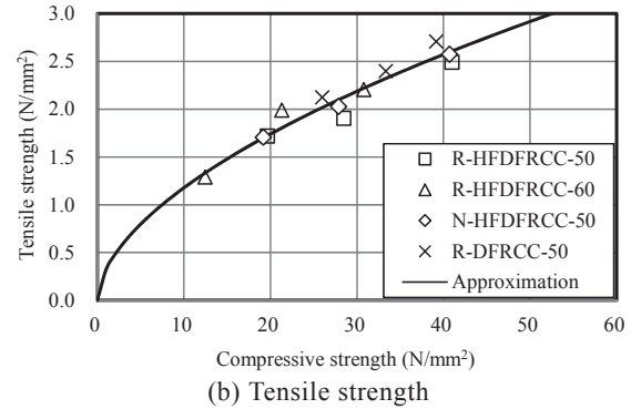
Fig.8 Flexural strength and tensile strength development.
