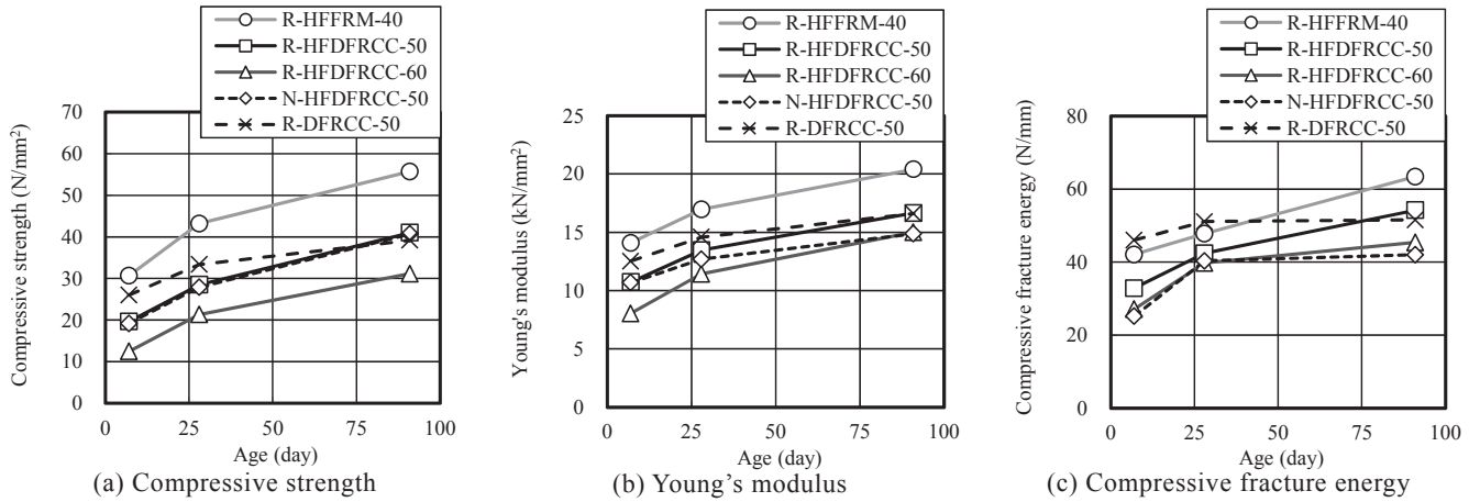
Fig.4 Compressive strength, young's modulus and compressive fracture energy – age relationship.
