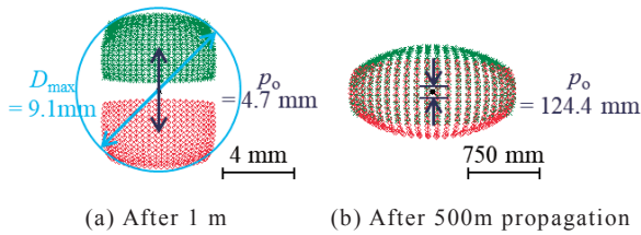
Fig. 5 Spot diagram
