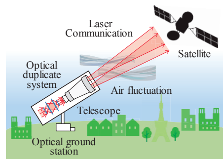
Fig. 1 Concept of satellite-ground laser communication
