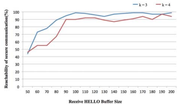
Fig.9 Reachability of secure communication
