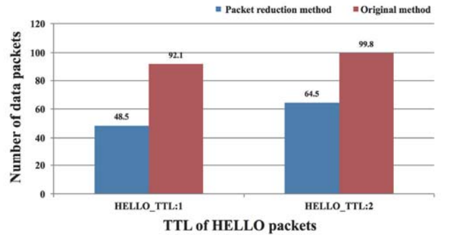
Fig. 12 Packet reduction effect
