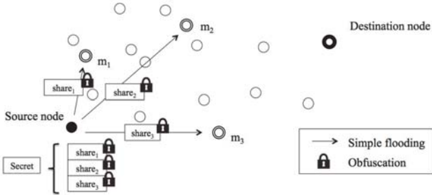
Fig.5 Transmission of obfuscated share data
