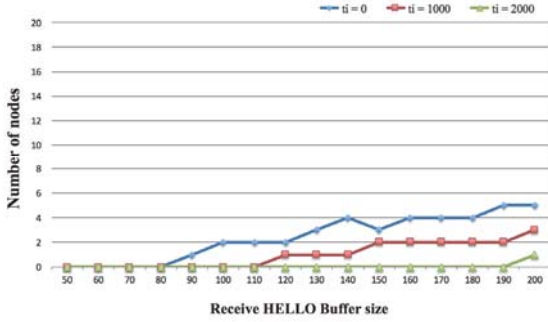
Fig. 10 Number of inappropriate nodes that capable of restoring a secret information
