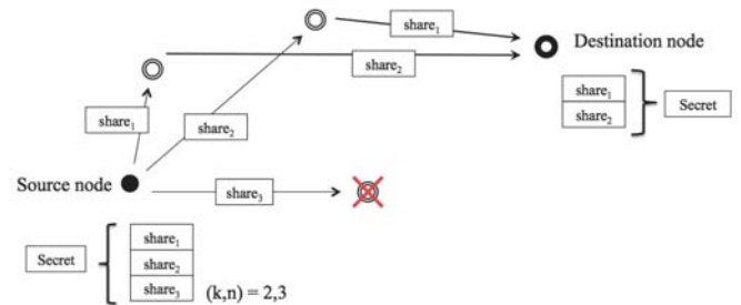
Fig.2 Secure communication method using (k, n) threshold scheme
