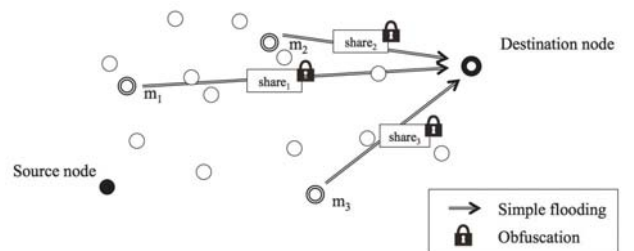
Fig.7 Obfuscated share data submission to destination by simple flooding
