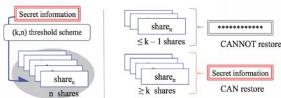
Fig.1 (k, n) threshold scheme
