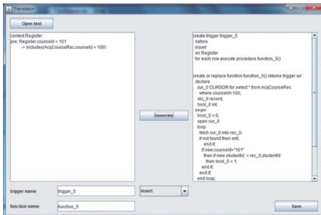
(b) GUI of OCL-trigger translator
