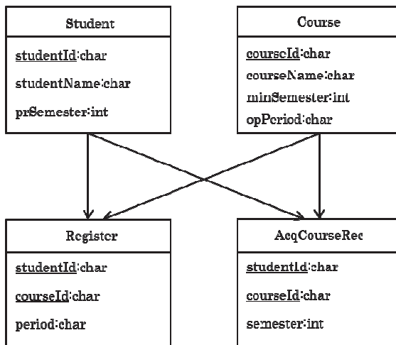
(b) Bachman diagram
