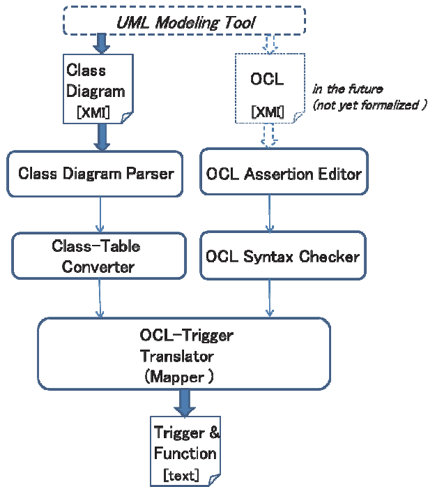
Fig.5 Activity of our tool.
