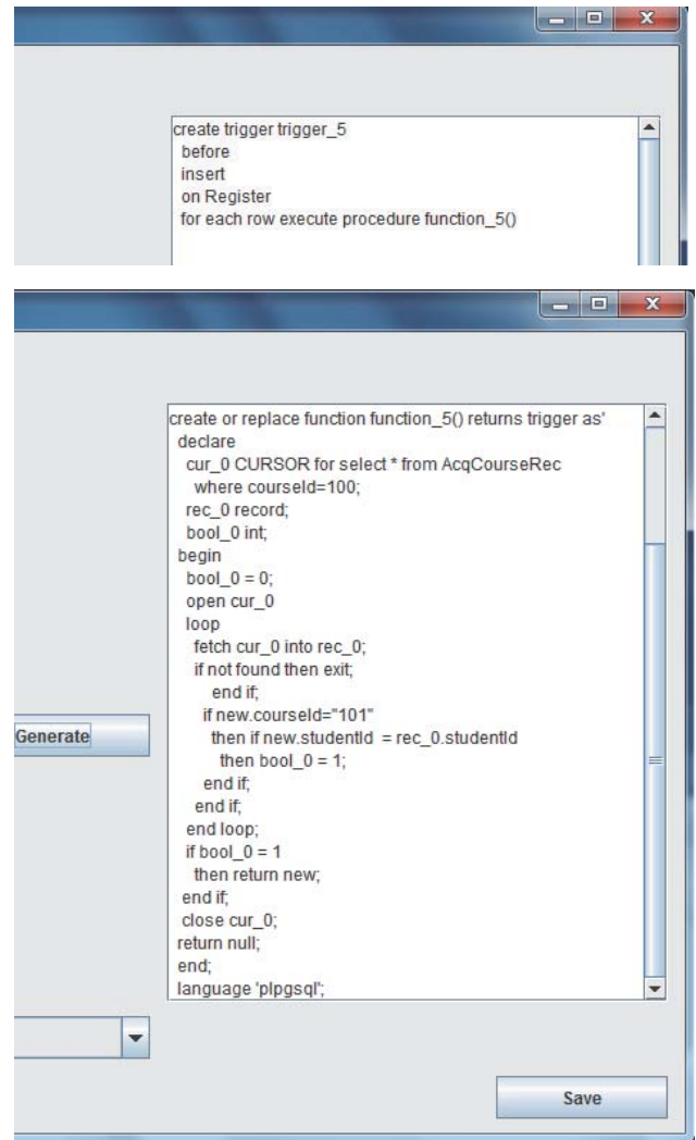
Fig. 8 Example of a transformation result.
