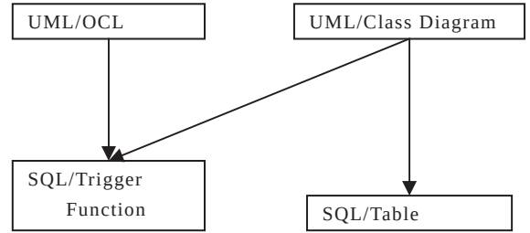
Fig.1 Transformation of assertion from OCL to trigger.
