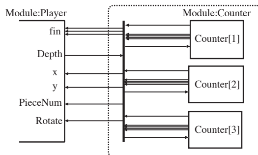
Fig.5 Multiple Counter Modules
