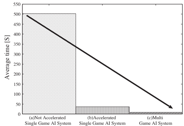
Fig.12 Average calculation speed of the systems
