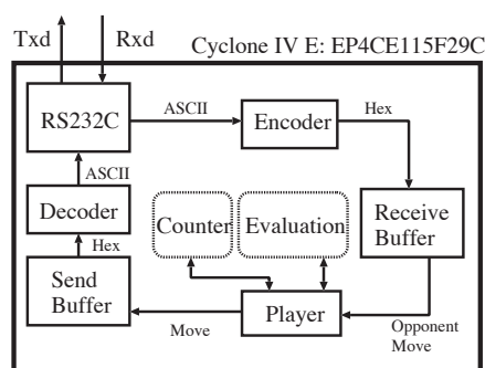
Fig.9 Block diagram of Single Game AI on FPGA
