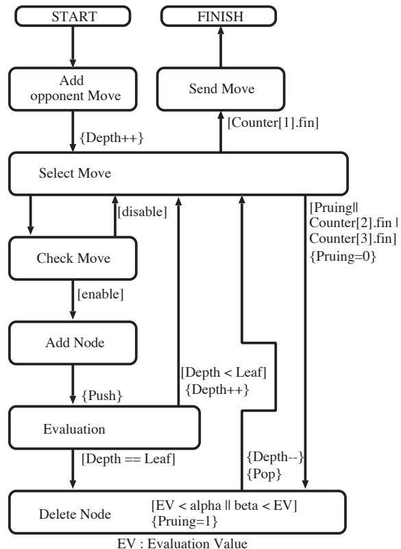
Fig.7 State transition diagram of Game AI
