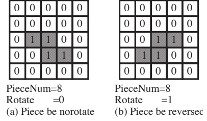
Fig.3 Example for rotate the pieces
