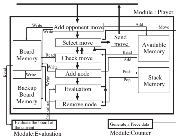
Fig.8 Block diagram of Player module
