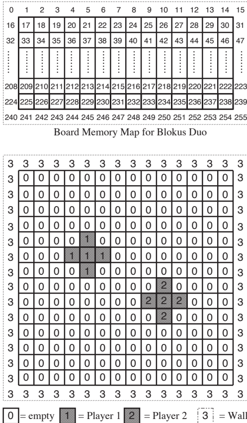
Fig.2 Index map of the board memory for Blokus Duo
