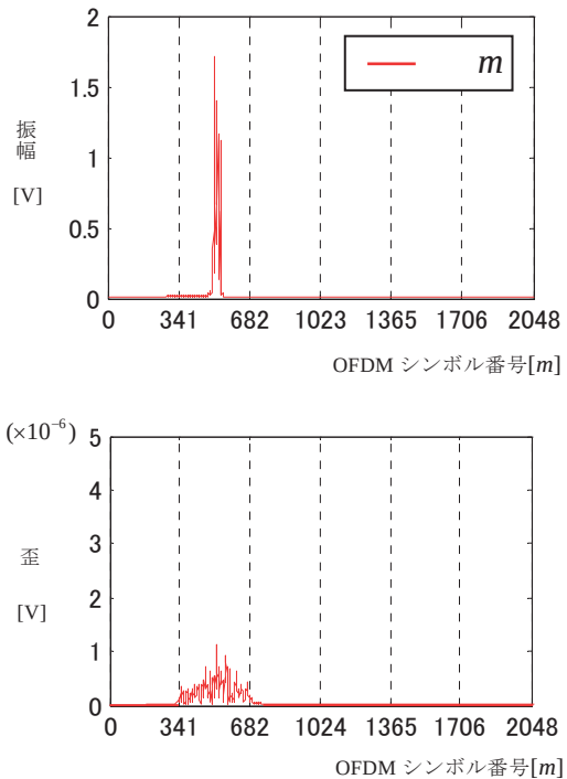
Fig.16 a e orm an istortion o estimate QAM signal ( sing raise cosine o trans er characteristic)
