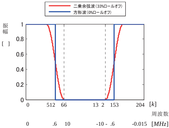
Fig.1 Transfer characteristics of 33 roll off
