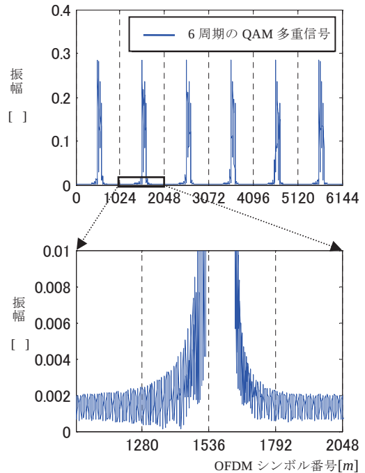
Fig.11 aveform of QAM signal of zero subcarrier
