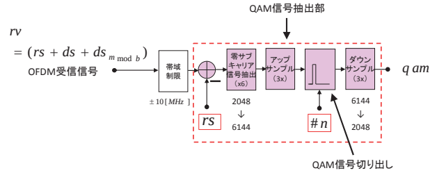
Fig.10 Block diagram of QAM signal extraction system
