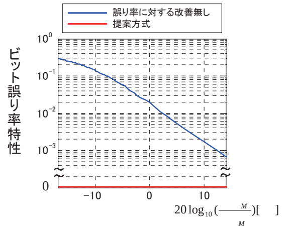
Fig.23 it error late o OFDM transmission system
