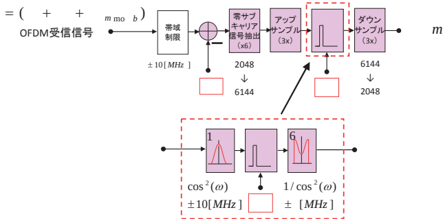
Fig.13 lock iagram o impro e system using s uare sine a e characteristic
