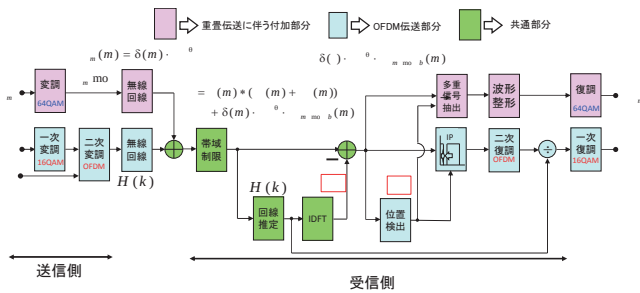
Fig.22 lock iagram o multiple transmission system o the OFDM signal an the QAM signal
