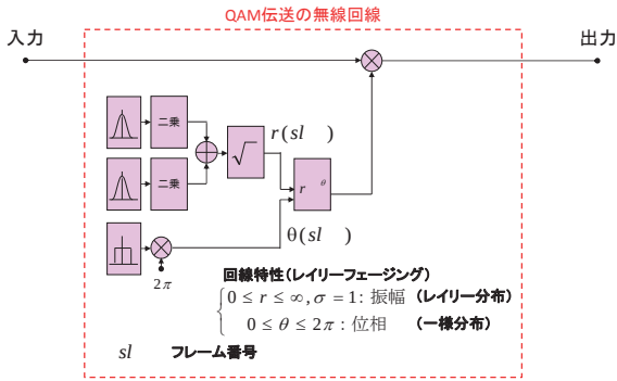
Fig. Block diagram of radio channel
