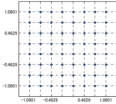
Fig.21 onstellation o 64 QAM emo ulator input signal
