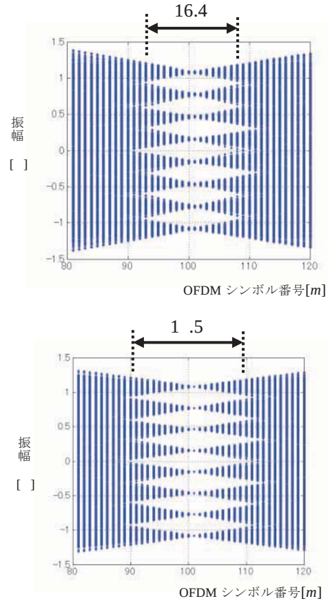
Fig.1 Eye pattern of using 0 roll off and 33 roll off characteristics
