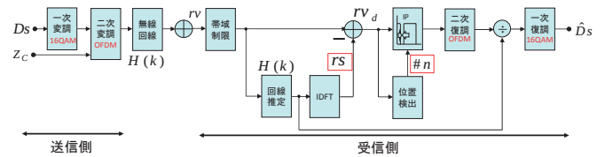
Fig.4 Block diagram of OFDM transmission system
