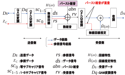
Fig.2 Structure of transmitter and receiver
