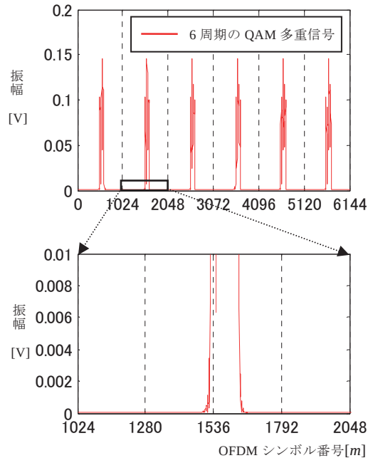
Fig.15 a e orm o QAM signal o zero subcarrier ( sing raise cosine o trans er characteristic)
