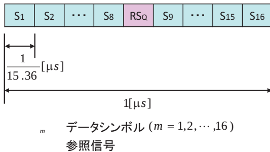
Fig. Frame composition of the transmission signal
