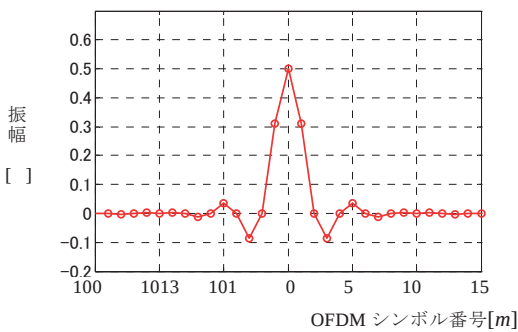
Fig.1 mpulse response (33 roll off)
