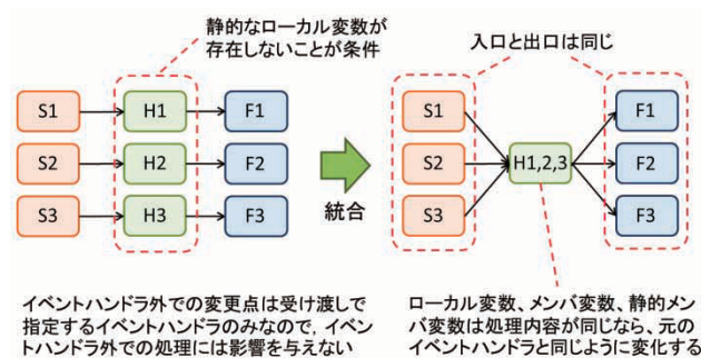
Fig.15 A change of calling way by the unified method
