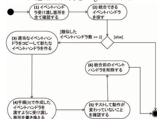
Fig.7 The process of unifying redundant event handlers
