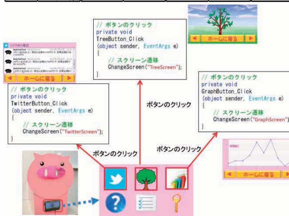
Fig.17 Redundant event handlers for screen transitions
