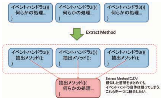
Fig.1 A problem of applying “Extract method”
