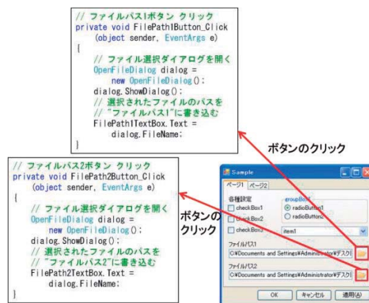
Fig.6 An example of specifying file path
