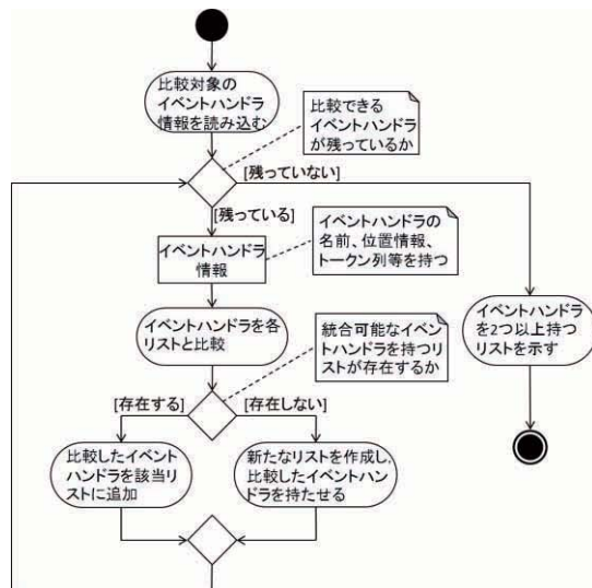
Fig.14 Constructing a list of event handlers for unifying
