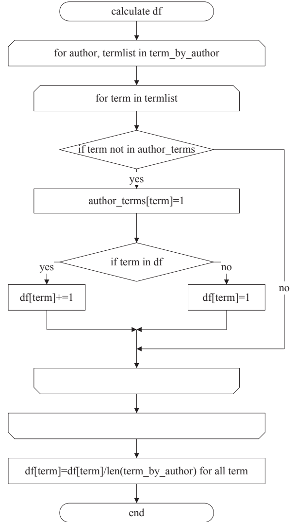
Fig. 2 Flow chart for calculating df parameter from extracted terms
