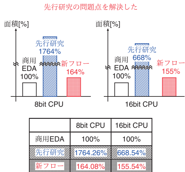
Fig.5 Area comparison of chips designed each method(commercial, previous research, new work)
