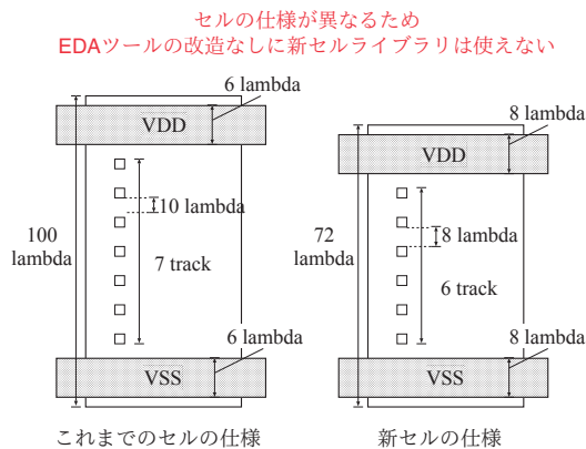
Fig.6 The cell specification difference
