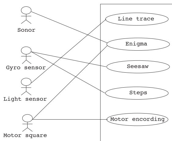
Fig.6 Usecase model
