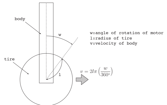
Fig.10 Velocity calculation of NXT
