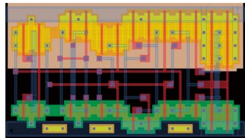
Fig.9 The adjusted examples of the layout
