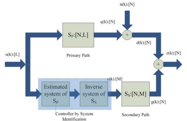
Fig.5 Proposed MIMO ANC system using system identification
