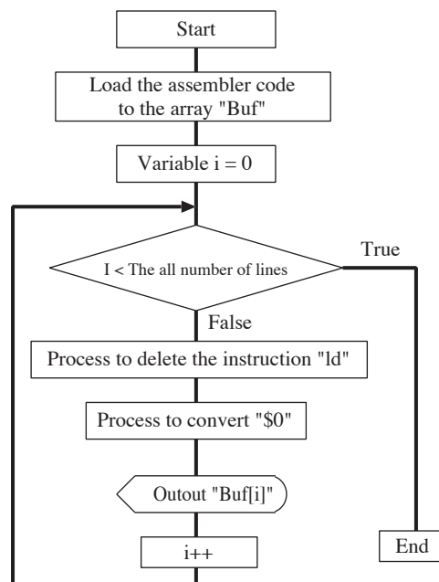
Fig4 Flow of assembler code optimization
