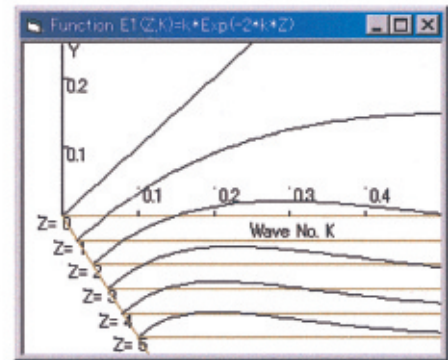
Fig. 3 Wave frequency and hydrofoil depth influence function.
