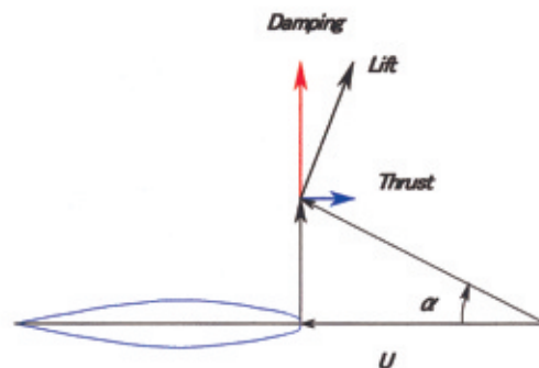
Fig. 1 Lift, thrust and damping force acting on the hydrofoil.
