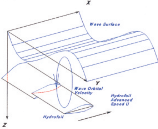
Fig. 2 Hydrofoil coordinates system and wave orbital velocity.
